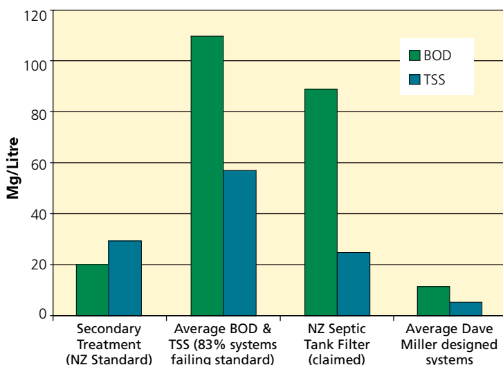
Hawkes Bay Region Sewage System Comparison {The lower the figure, the better the treatment}
