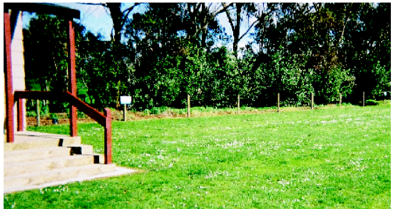
The treated effluent disposal area in shelter belt along fence line. (The effluent is treated to a quality 5 times better than required by the NZ Standards and 20 times better than the quality produced by 83% of the treatment systems tested in the Hawkes Bay Monitoring program).
